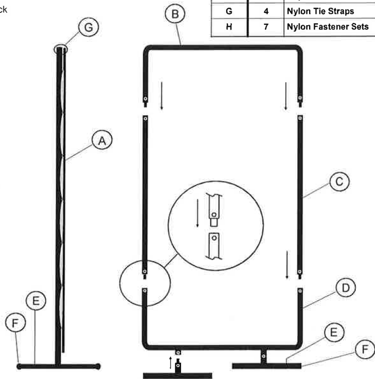
SNAP-LOCK FRAME ASSEMBLY
