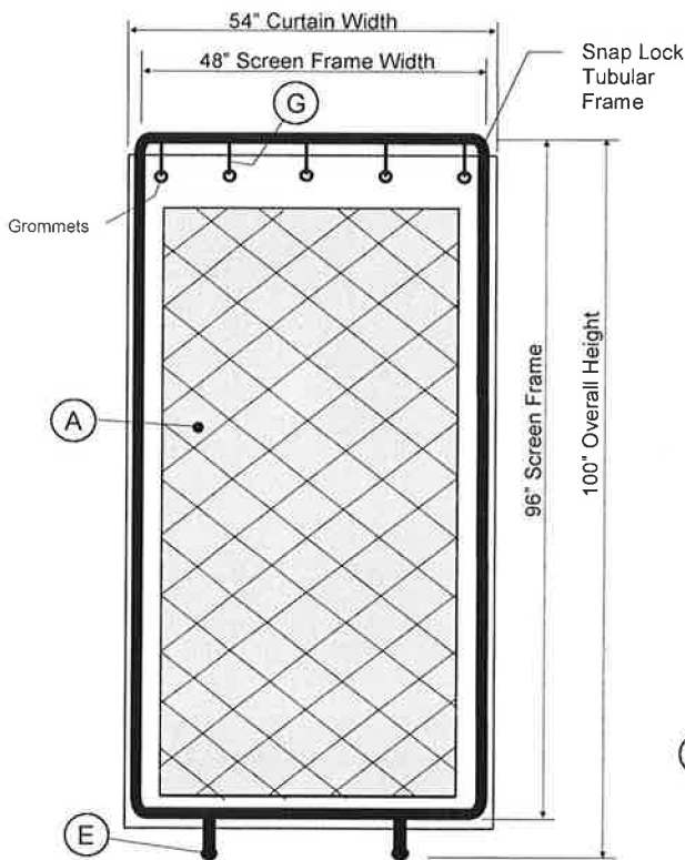
STANDARD SCREEN ASSEMBLY Shown With Composite Curtain
