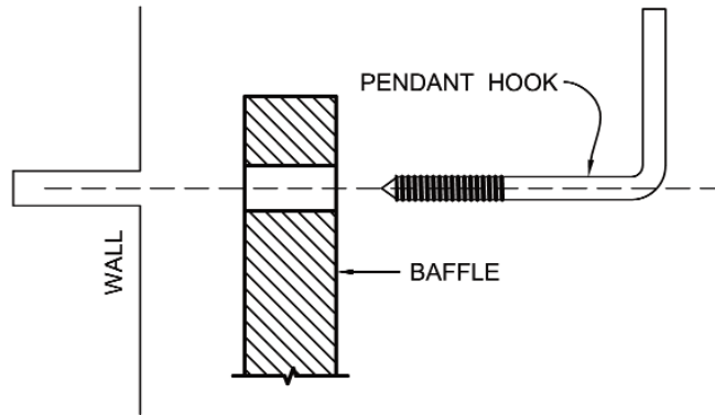
A ATTACHMENT DETAIL CL-6 CL-6 SCALE: NA
