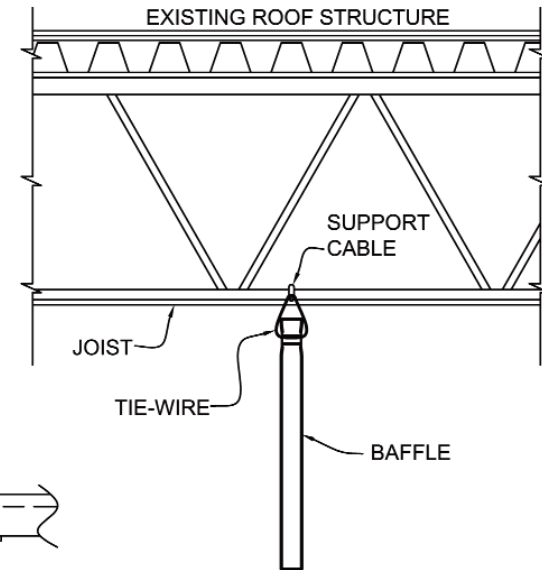
SIDE ELEVATION
